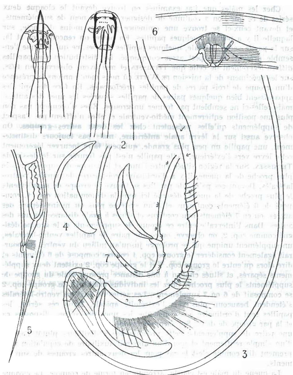
FIG. 2b. — Actinolaimus omer-cooperi FILIPIEV.
