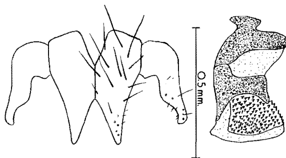
FIG. 43. — Mitlogramma helvum VILLENEUVE. Cerci with paralobi and phallosome. (Specimen from Oudtshoorn, Cape Province.)
