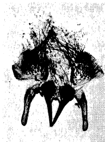
FIG. 5. — Termitometopia skaipei ZUMPT. Microphotograph of cerci with paralobi and of phallosome. (Paratype from Cape Town.)
