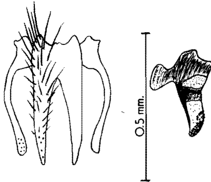
FIG. 16. — Senotainia ravilla n. sp. Cerci with parolobi and phallosome. (Holotype from Salisbury, S. Rhodesia.)
