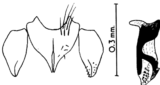
FIG. 47. — Apodacra stevensoni n. sp. Cerci with paralobi and phallosome. (Specimen from Bulawayo, S. Rhodesia.)
