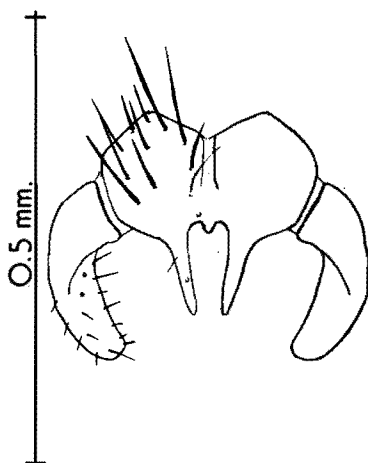
FIG. 33. — Taxigramma biseta (VILLENEUVE). Cerci with paralobi. (Specimen from Mamathes, Basutoland.)
