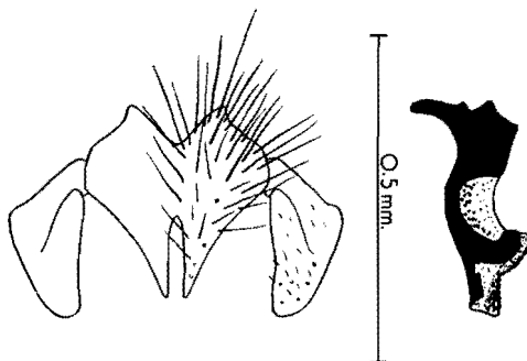
FIG. 27. — Metopia deficiens VILLENEUVE. Cerci with paralobi and phallosome. (Specimen from Hout Bay, Cape Peninsula.)
