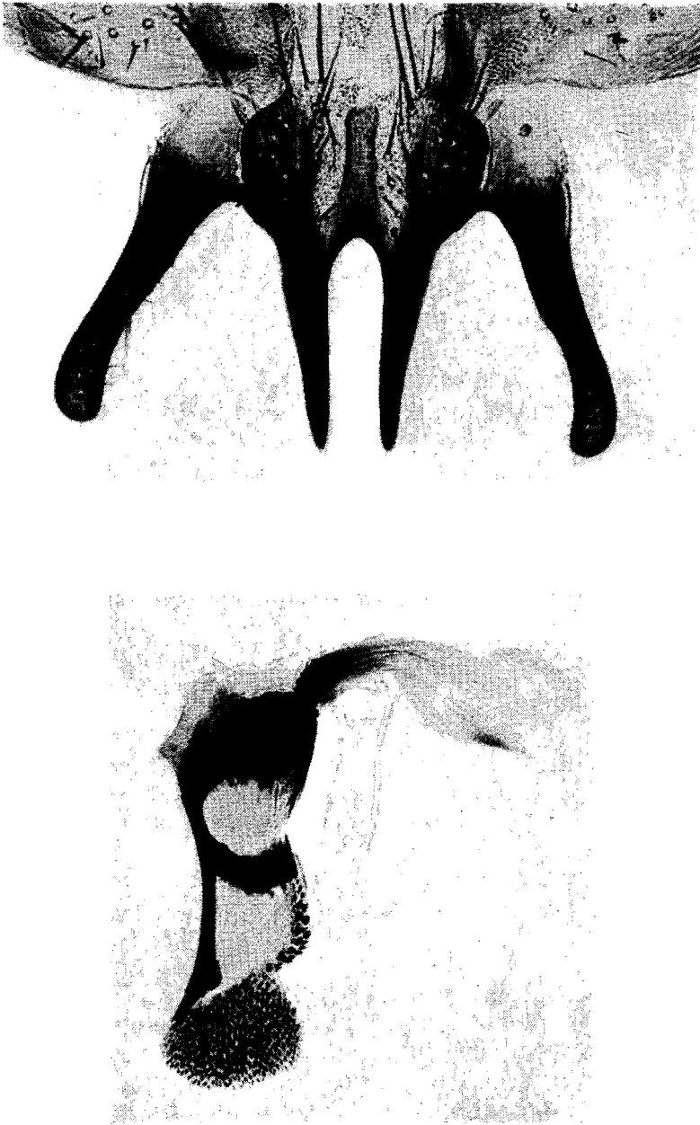
FIG. 30. — Metopodiella eos n. sp. Cerci with paralobi and phallosome. (Paratype from Victoria, S. Rhodesia.)
