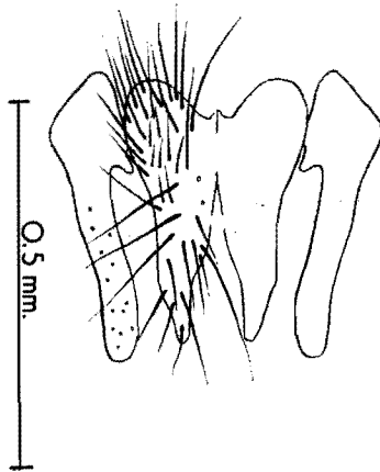
FIG. 23. — Paraphylloteles hessei ZUMPT. Cerci with paralobi. (Holotype from Spitzkop, Cape Province.)
