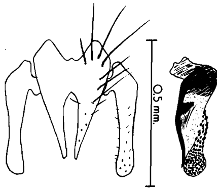
FIG. 7. — Hoplatania pilosa n. sp. Cerci with parolobi and phallosome. (Holotype from Pretoria, Transvaal.)
