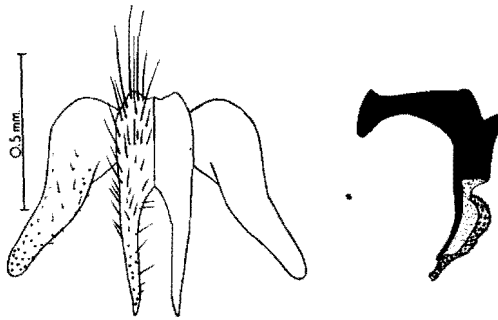
FIG. 1. — Hoplancephala retroseta VILLENEUVE. Cerci with paralobi and phallosome. (Specimen from Johannesburg, Transvaal.)
