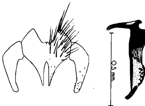
FIG. 46. — Miltogramma munroi CURRAN. Cerci with paralobi and phallosome. (Paratype from Barberton, Transvaal.)
