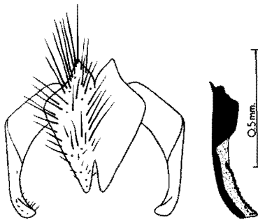
FIG. 45. — Millogramma hirtimanum BEZZI. Cerci with paralobi and phallosome. (Specimen from Mayumbe, Congo.)
