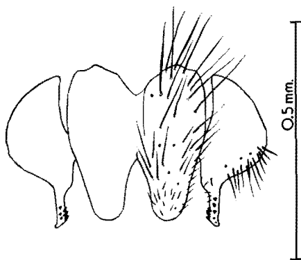
FIG. 21. — Noditermitomyia currani n. sp. Cerci with paracymbria. (Holotype from Salisbury, S. Rhodesia.)
